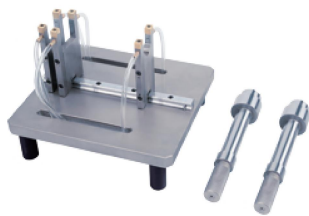
single-section air ring outside diameter measuring stages and standard gauges
