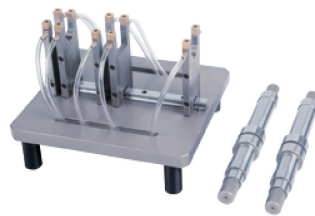
air angle gauges and standard gauges
