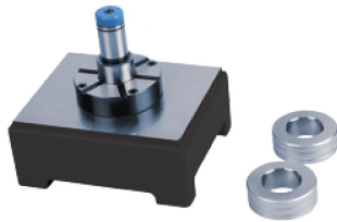
three-section air outside diameter measuring stages and standard gauges
