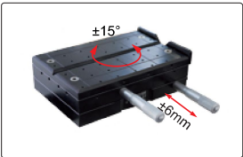
stage (included)
